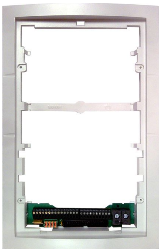
Adapter-Rahmen CL-888-58M-01
